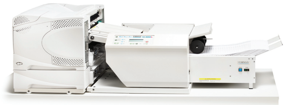
FD 2052IL System shown with IL Pressure Sealer and IL Alignment Base, laser printer (not included), optional conveyor and optional locking cabinets
